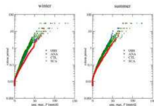
Fig. 3 Return periods for extreme precipitation. The large spread for the strong events, i.e. the major source of uncertainty, arises from natural fluctuations - as simulate by CTL . The model error (= difference between OBS and ANA/CTL ) is relatively small. A significant increase exists for moderate return periods of about 1 y, especially for winter (left panel).
