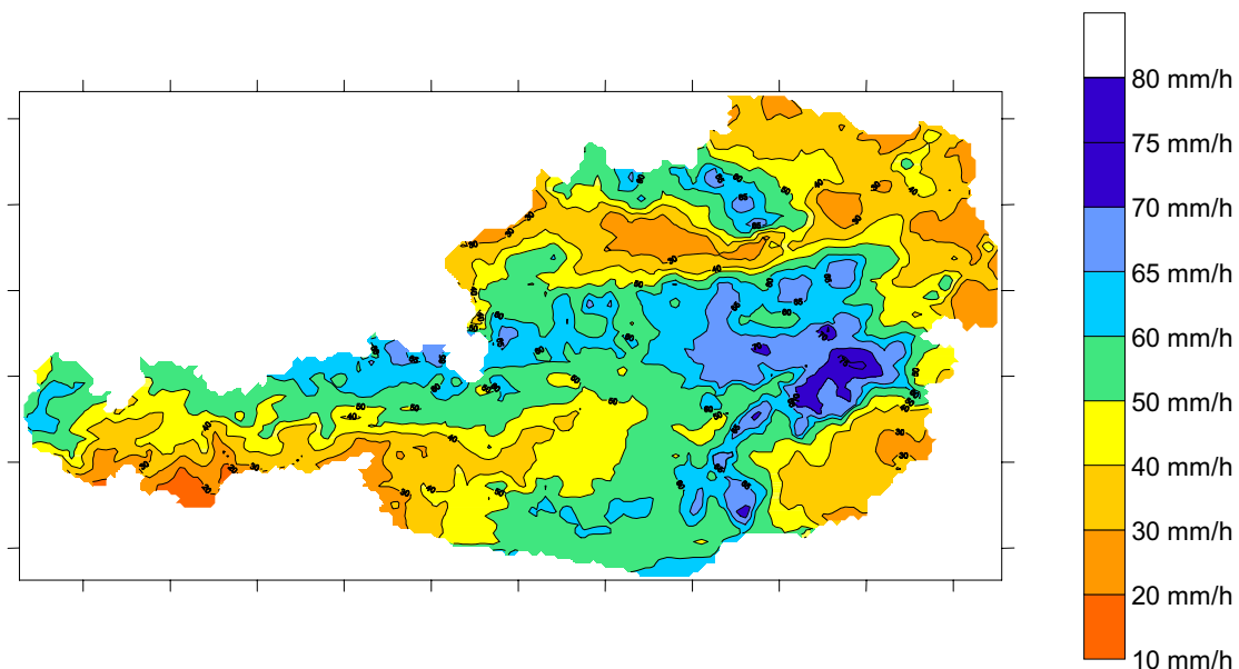
Fig. 4 Design values of maximum precipitation in Austria for D = 3 \text{ h} and T = 100 \text{ a} .
