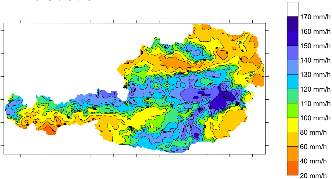
Fig. 3 Design values of maximum precipitation in Austria for D = 1 \text{ h} and T = 100 \text{ a} .
